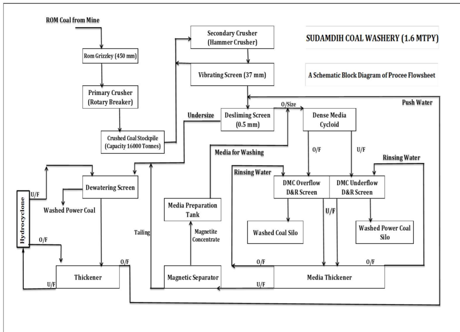
Existing Flow Sheet of Sudamdih Coal Washery
